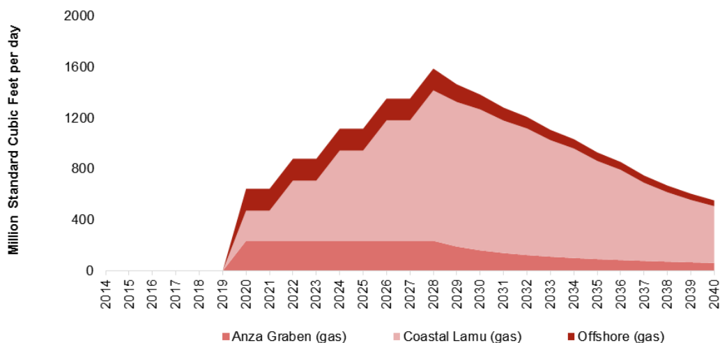
Figure 4.6: Base case gas supply profiles
