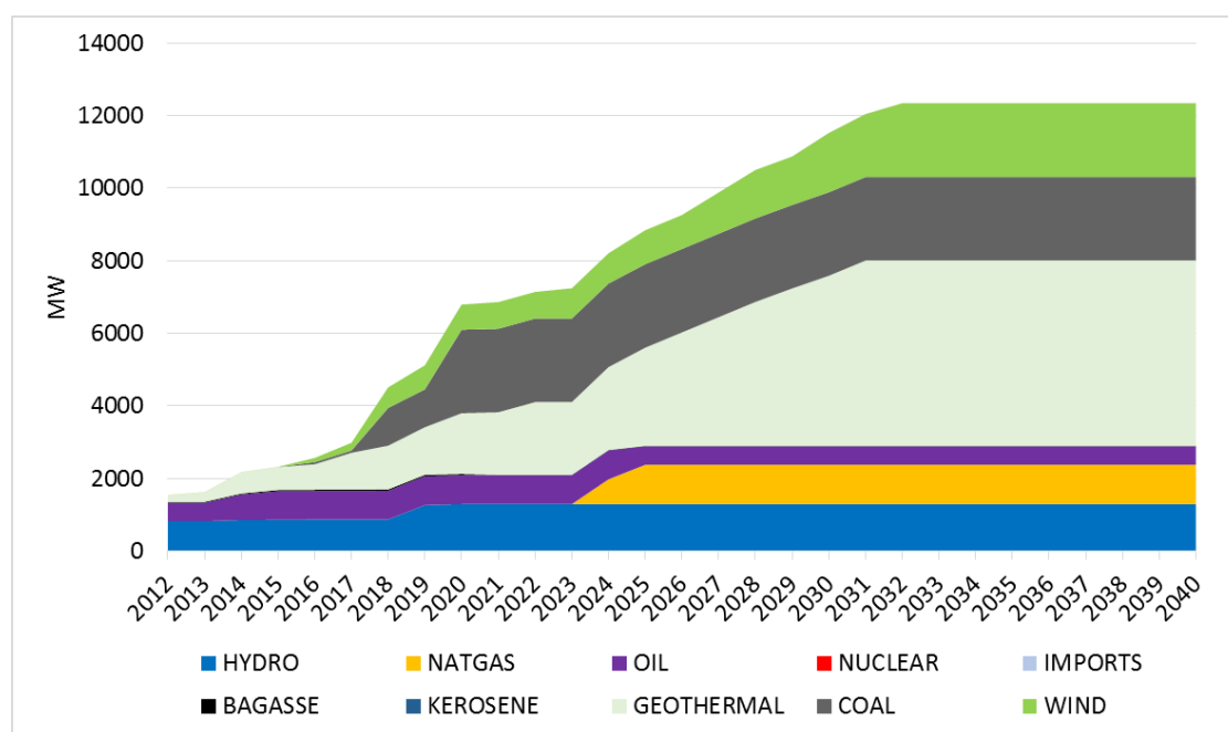
Figure H – 2: Power generation forecast – Low case
