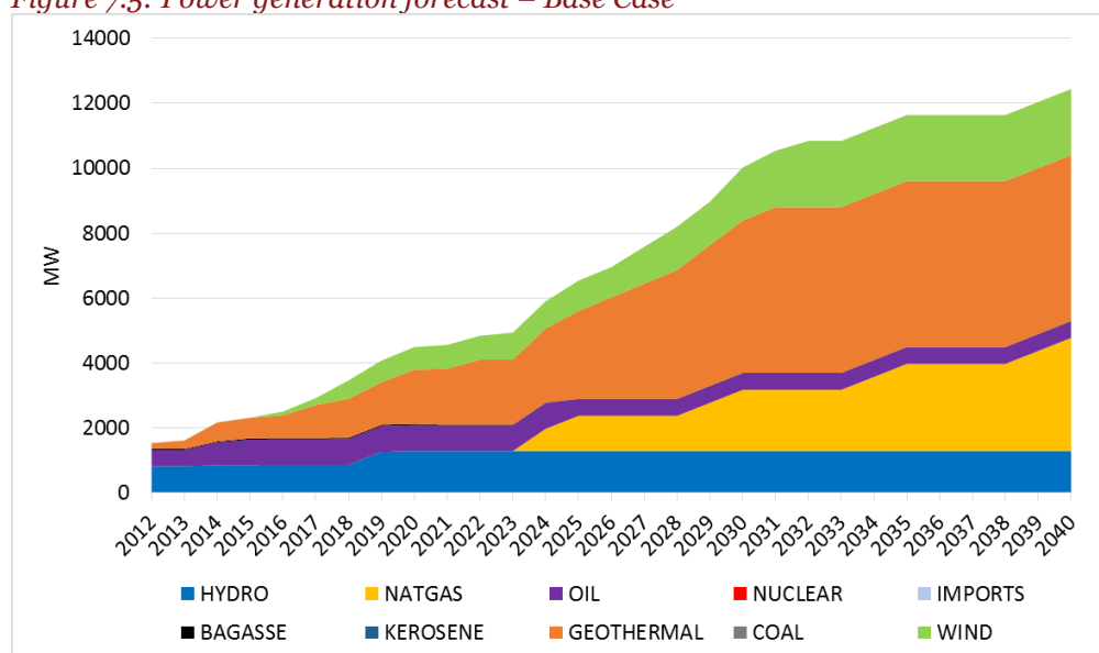
Figure 7.5: Power generation forecast – Base Case
