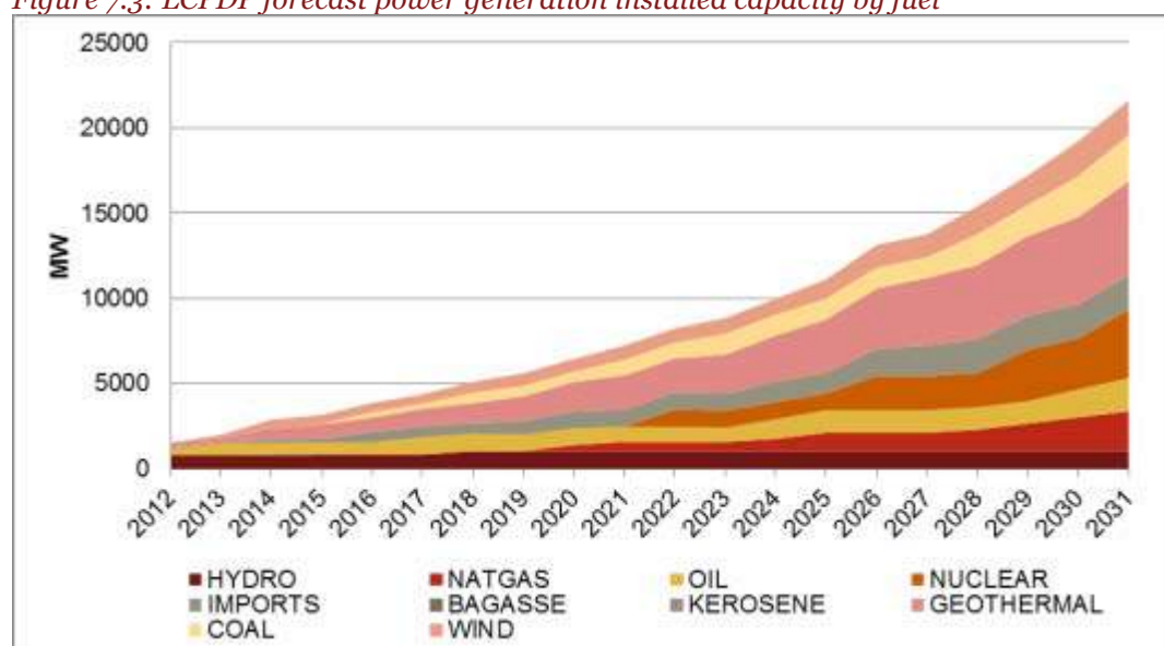
Figure 7.3: LCPDP forecast power generation installed capacity by fuel
