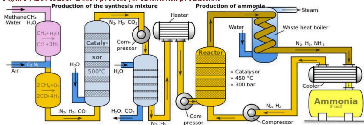
Figure 7.20: Haber-Bosch process for Ammonia production
