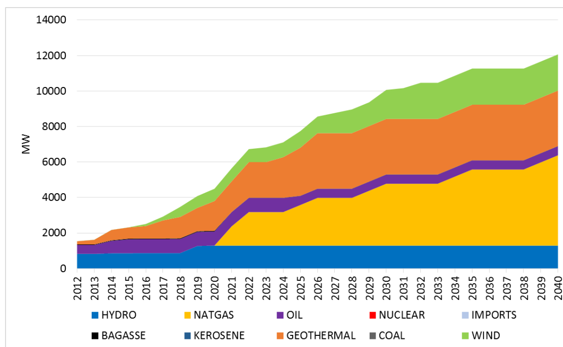
Figure H – 3: Power generation forecast – High case
