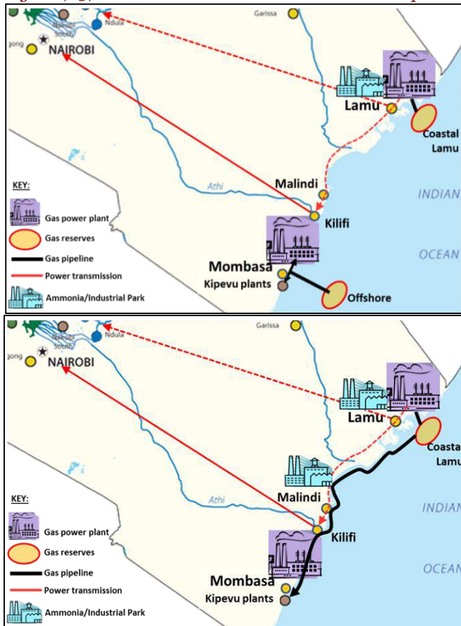
Figure 7.37: Scenario 1: Base case coastal CCGT plant development and power transmission
