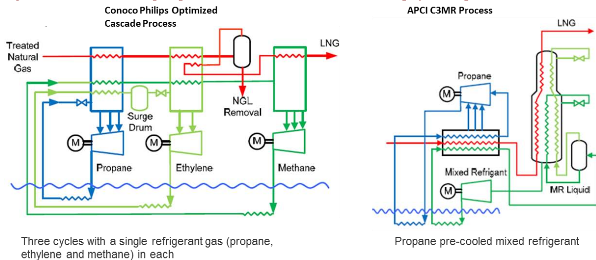
Figure 7.30: Conoco Philip's optimised cascade and APCI's C3MR liquefaction process
