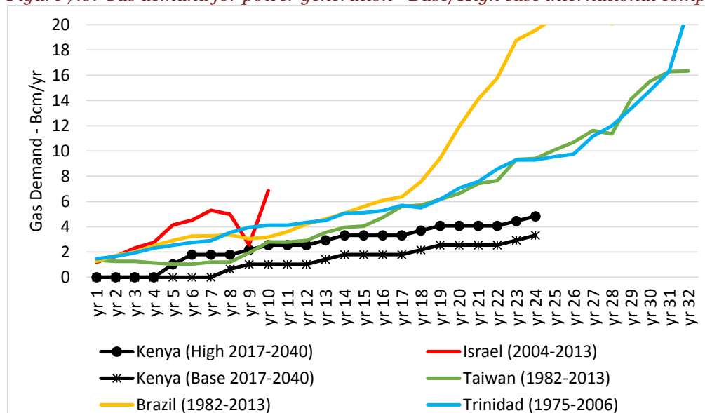
Figure 7.6: Gas demand for power generation - Base/High case international comparisons
