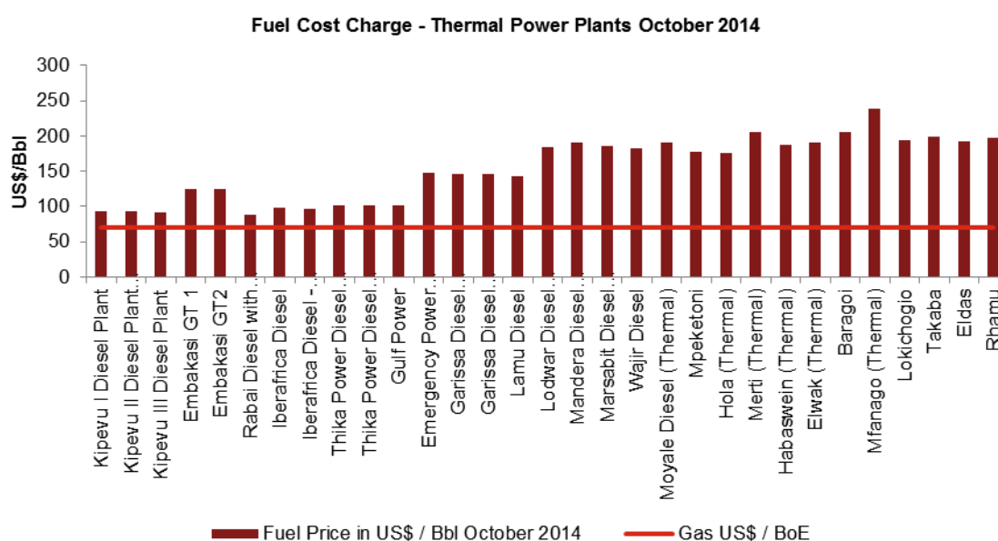
Figure 7.10: Fuel cost charge of thermal power generation, 2014
