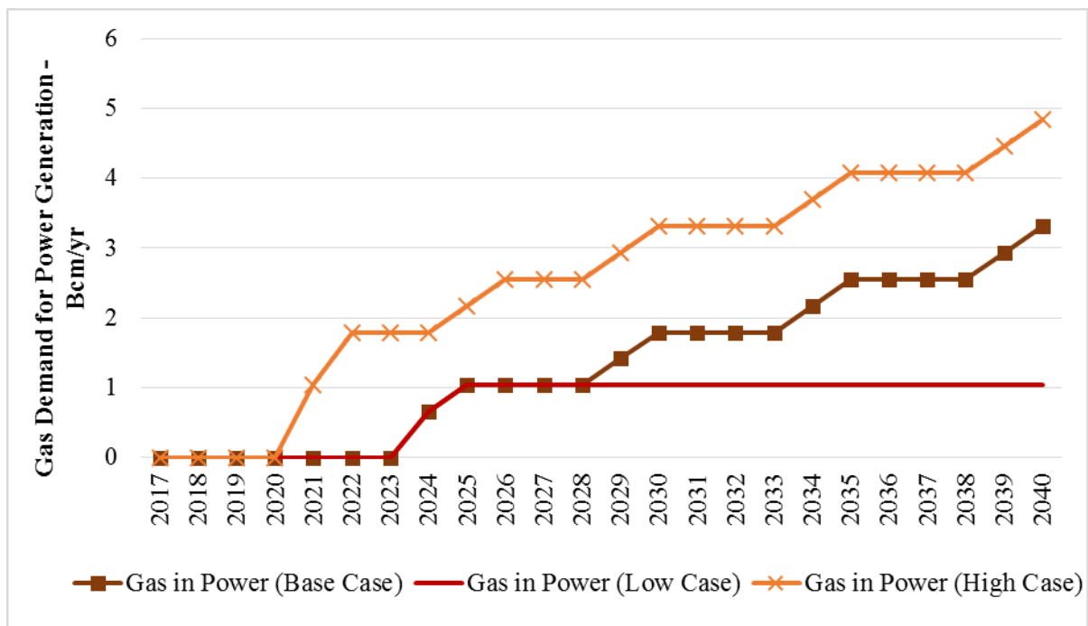
Figure H – 4: Gas demand in power generation – all scenarios
