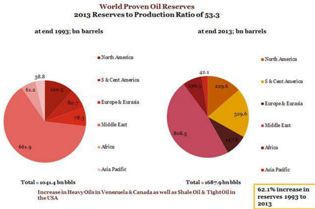
Figure F – 2: Global oil reserves – 1993 & 2013
