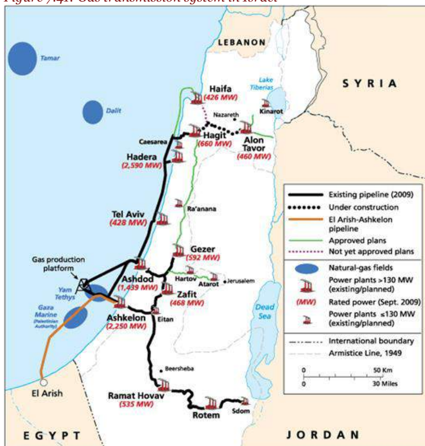
Figure 7.41: Gas transmission system in Israel
