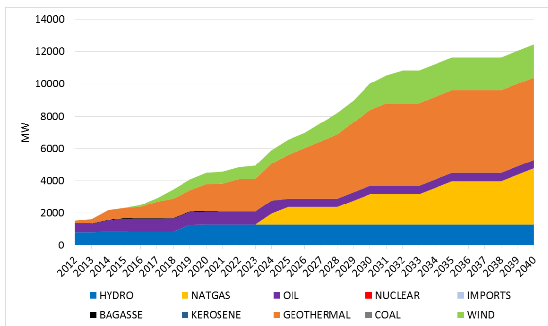
Figure H – 1: Power generation forecast – Base case
