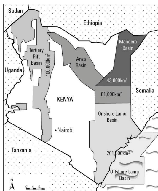
Kenya basins structural framework
