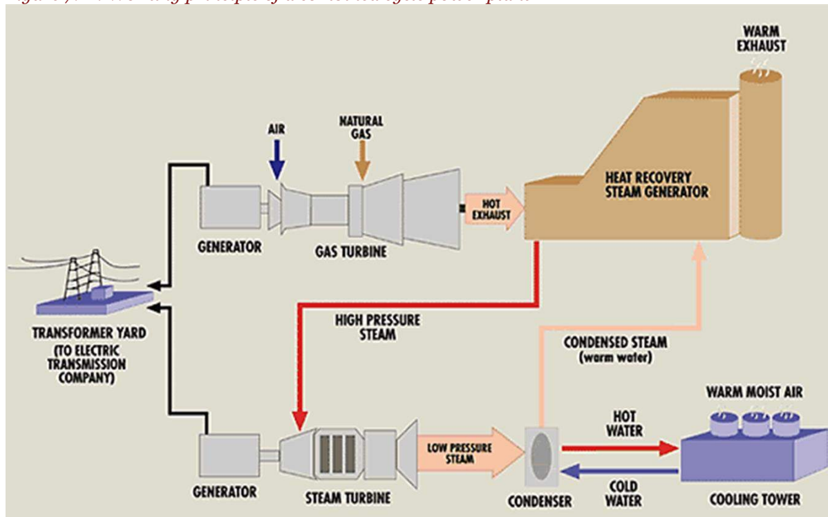
Figure 7.12: Working principle of a combined cycle power plant
