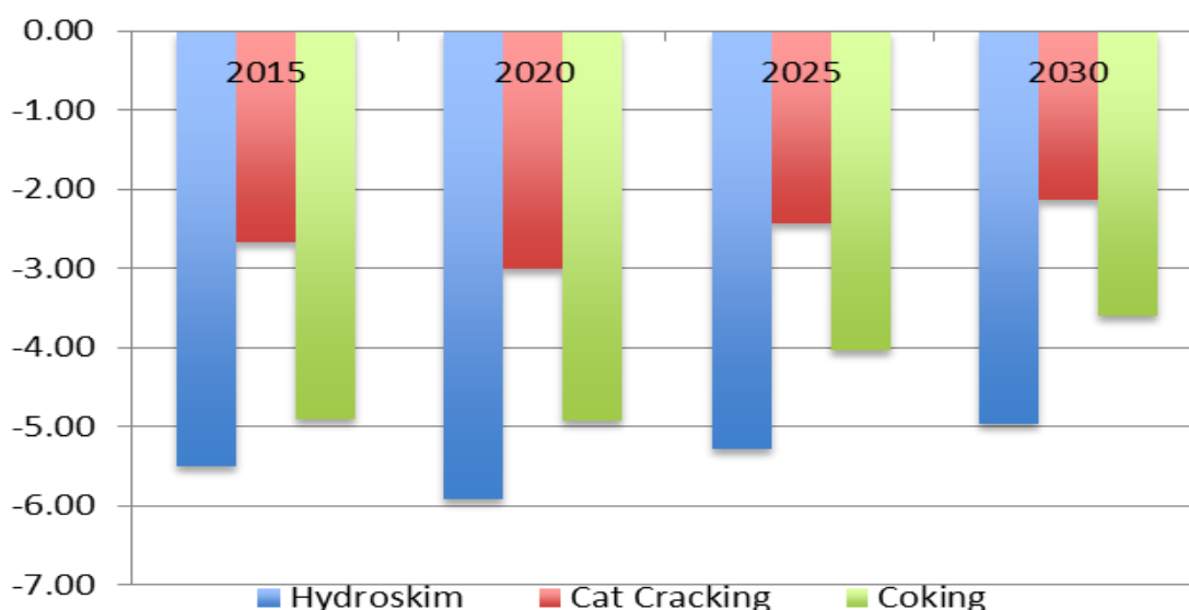
Figure 6.11: Full cost margins (*WACC 10%) on 200 kb/d (US$/bbl)
