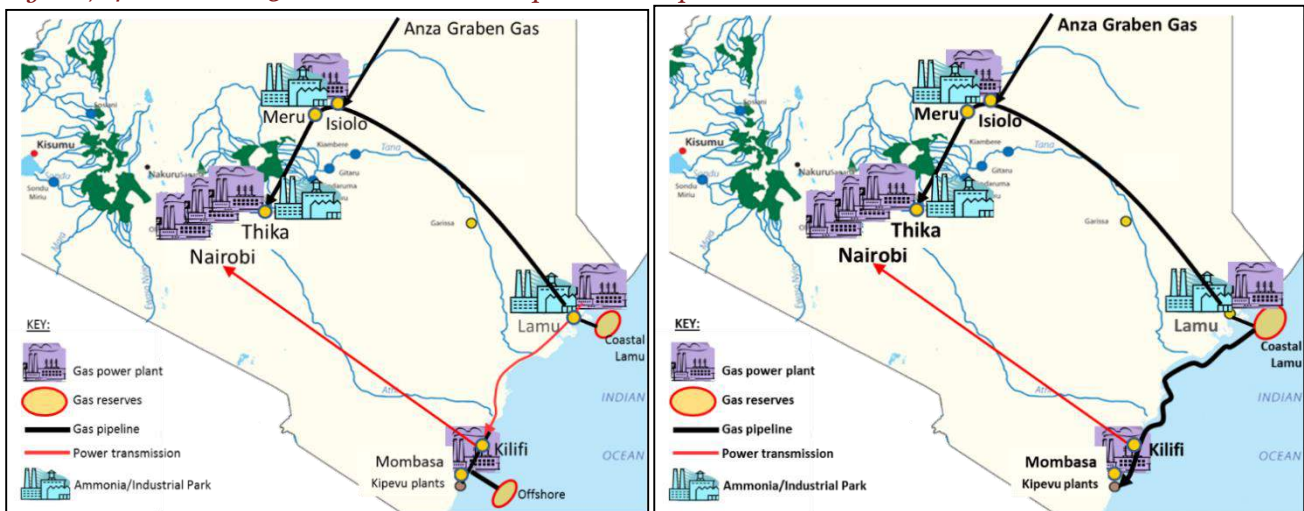
Figure 7.40: Scenario 3: Coastal and inland plant development
