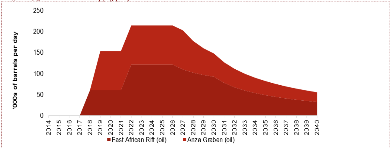
Figure 4.5: Base case oil supply profiles
