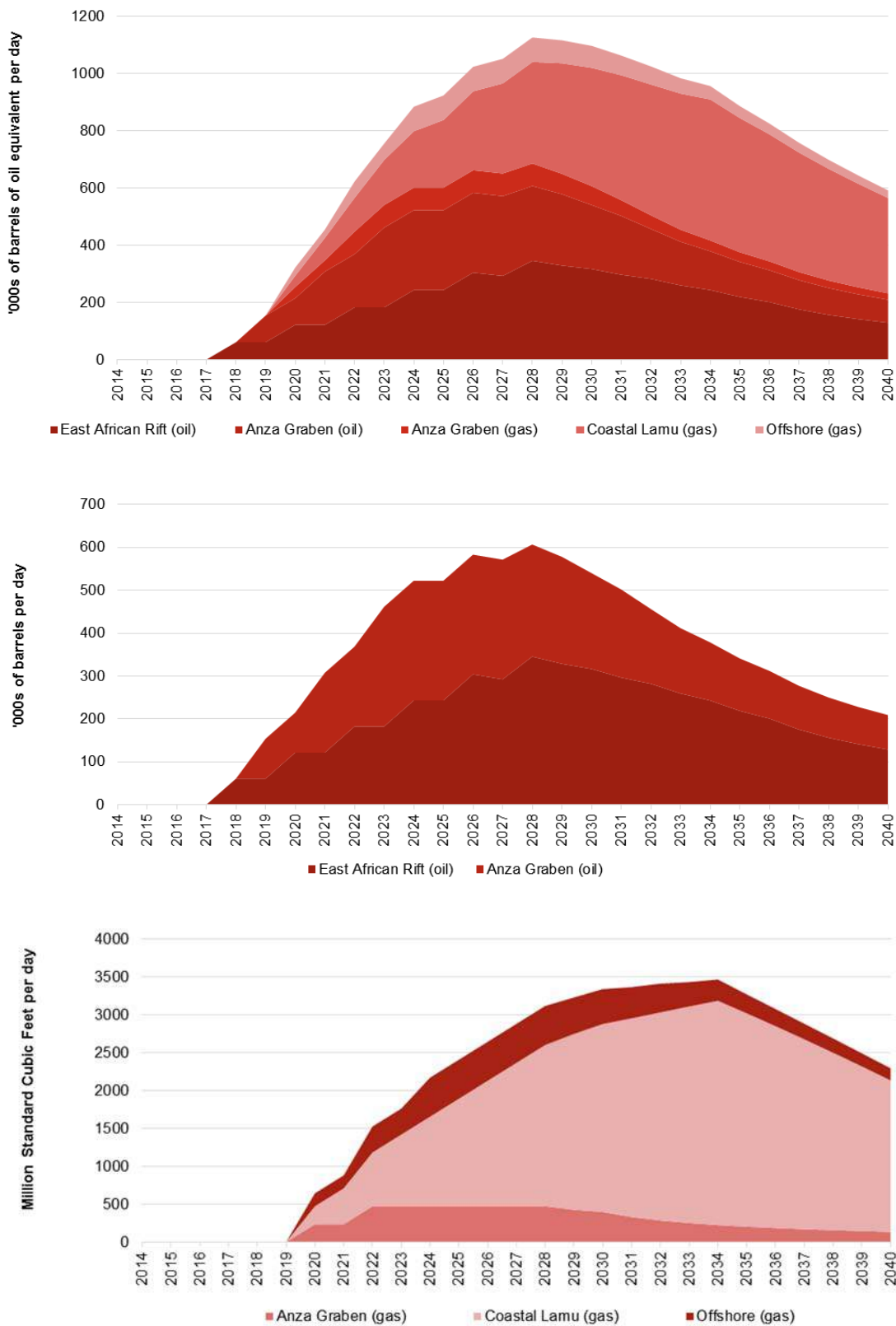
Figure E - 1: High case oil and gas supply profiles
