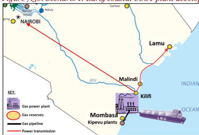
Figure 7.36: Scenario 1: Early coastal CCGT plant development and power transmission
