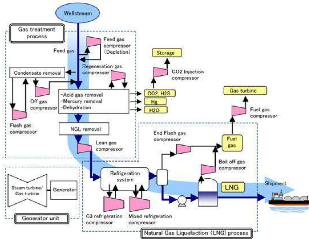
Figure 7.29: Overall LNG production process
