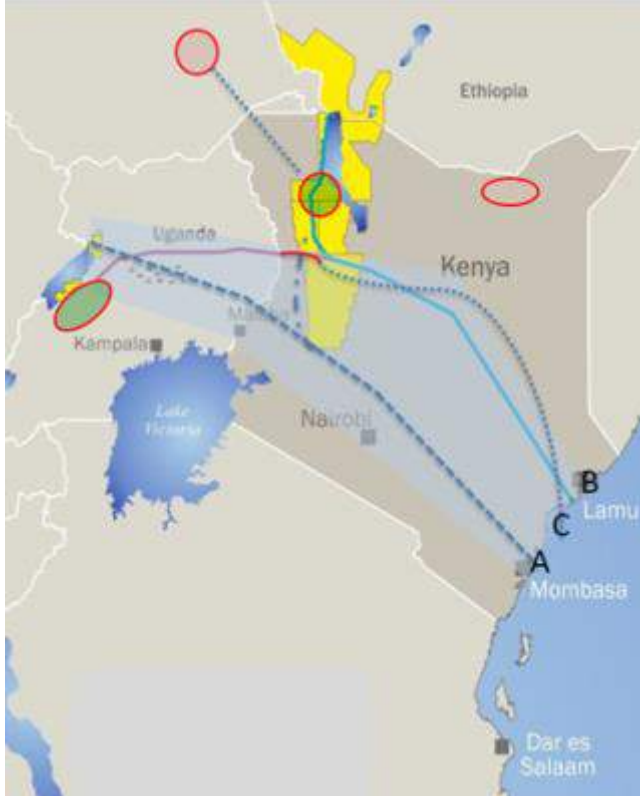
Figure 5.4: Crude oil export pipeline – routing options
