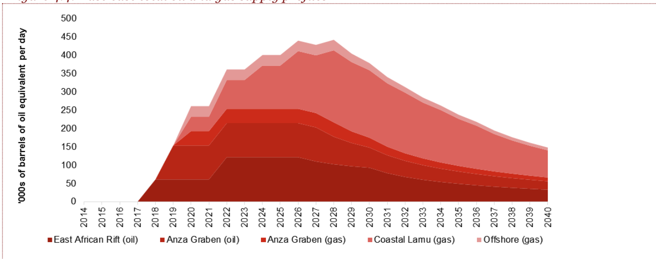
Figure 4.4: Base case total oil and gas supply profiles
