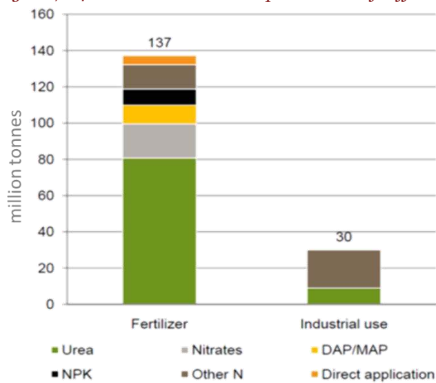
Figure 7.14: Ammonia use in the production of different products
