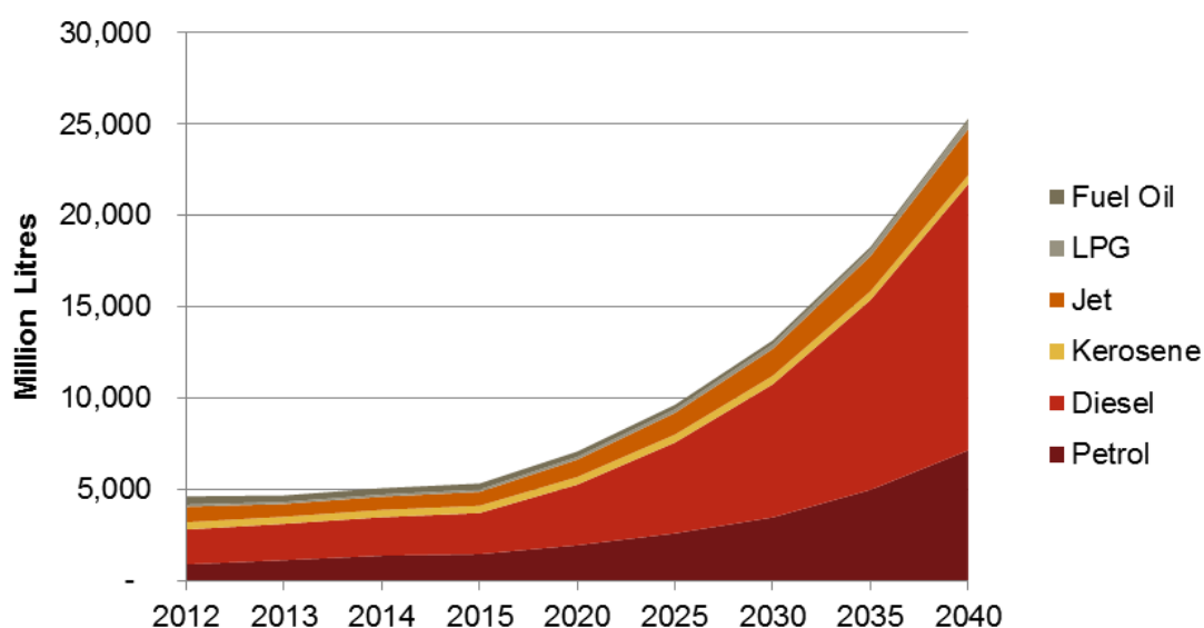
Figure F -13: Base-case projections
